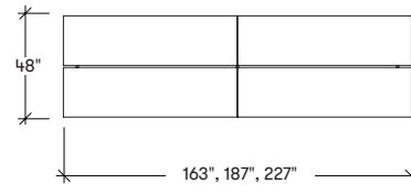
Rec Ganged Single Top Workshop Tables STMB
