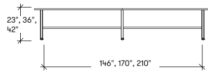
Rec Ganged Single Top Workshop Tables STMB
